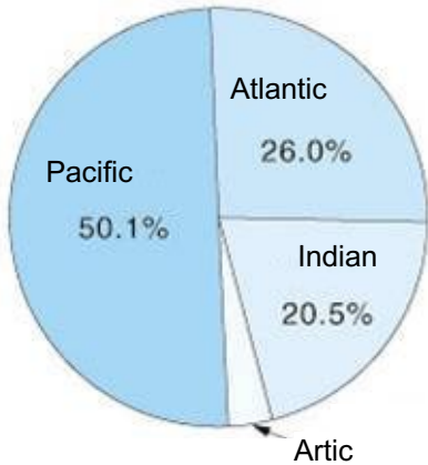
relative dimensions of the oceans
