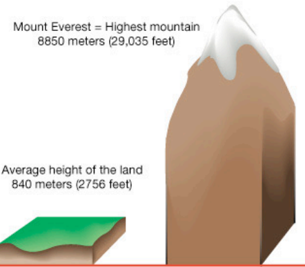
Depth of oceans and altitude of continents
